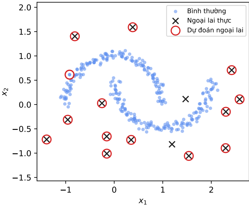
Autoencoder (MLP) — 2-8-2-8-2, loss=0.00058
